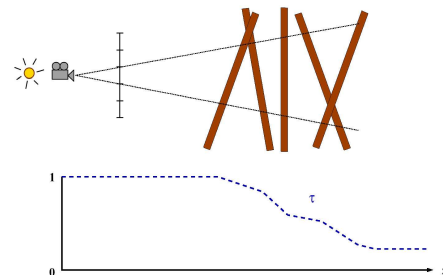
Fig. 24. Top: a beam of light starting at the shadow camera origin ( i.e. , the light source) and passing through a single pixel of the deep shadow map. Bottom: the corresponding transmittance (or visibility) function \tau , stored as a piecewise linear function.
