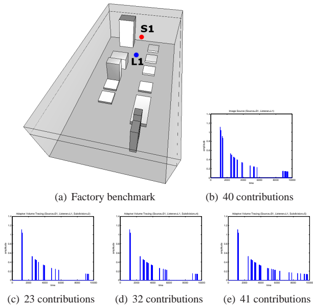
Fig. 10. (a) Factory benchmark with 174 triangles. (b) Impulse response generated by image source method for 3 reflections. (c)–(e) Impulse responses generated by our approach with maximum sub-division depth of 2, 4, and 5 respectively for 3 reflections.
