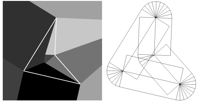
Figure 4: The per-feature Voronoi diagram of a quadrilateral (left). The corresponding distance mesh (right).
