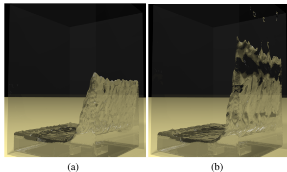
Figure 6: Dam Break example at t=0.48s using PIC(left) and FLIP(right) showing maximum height reached by water
