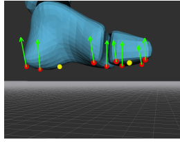
(b) Contact points (red) and contact forces (green) on a foot.
