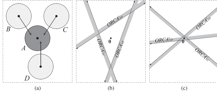
Fig. 5 (a) A dense configuration with three robots moving towards robot A . The current velocities of the robots are shown using arrows; robot A has zero velocity. (b) The half-planes of permitted velocities for robot A induced by each of the other robots with \tau = 2 and \mathbf{v}_*^{\text{opt}} = \mathbf{v}_* for all robots. The region ORCA_A^\tau is empty, so avoiding collisions within \tau time cannot be guaranteed. (c) The half-planes of permitted velocities for robot A induced by each of the other robots with \tau = 2 and \mathbf{v}_*^{\text{opt}} = \mathbf{0} for all robots. The dashed region is ORCA_A^\tau .
